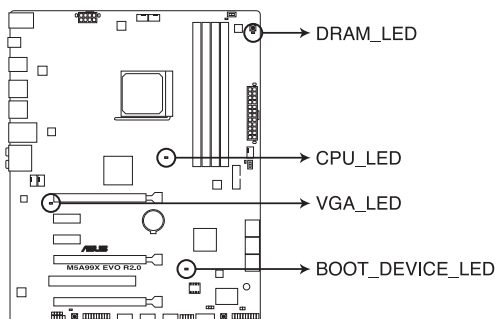
LED du POST de la M5A99X EVO R2.0
