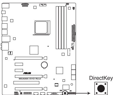
Bouton DirectKey de la M5A99X EVO R2.0
